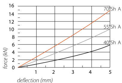
Load Fz
