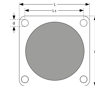
Crane buffer with base plate
