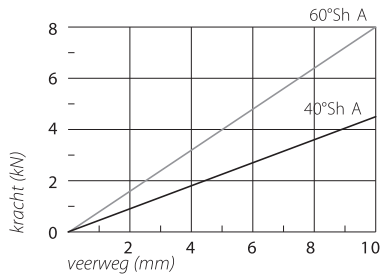
Belasting Fz
