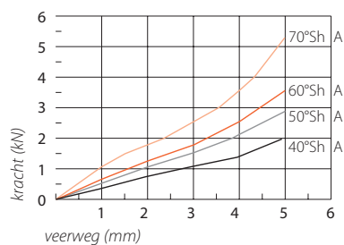
Belasting F_z
