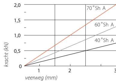
Belasting Fx, Fy
