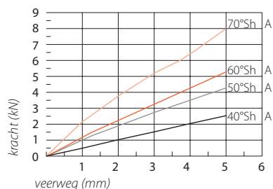
Belasting Fz
