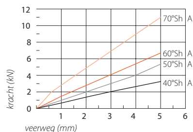
Belasting Fz
