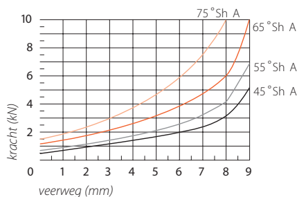
Belasting Fz
