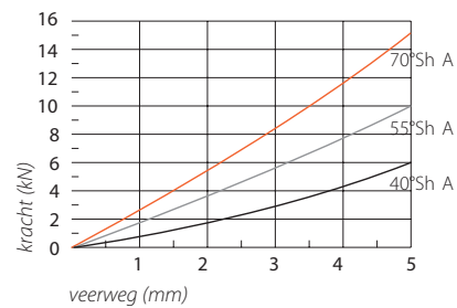
Belasting Fz
